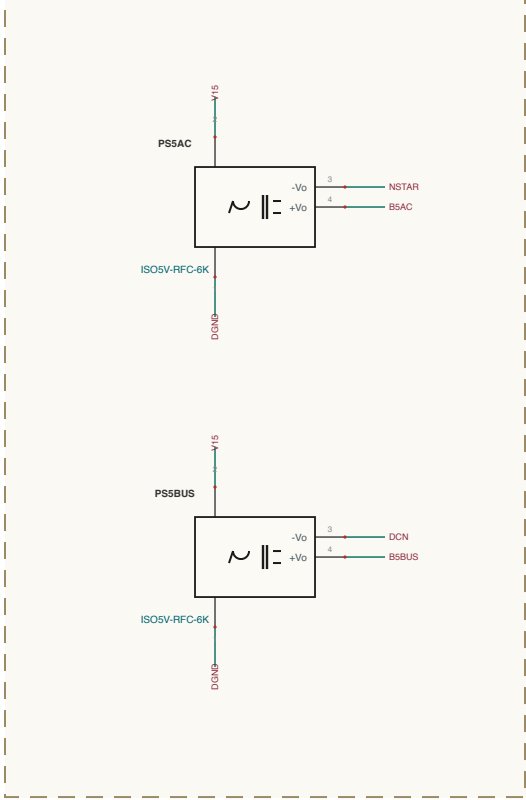
AC-SENSING / ISO-BIAS
