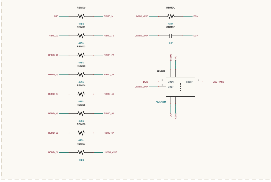
AC-SENSING / SENSE-VMD
