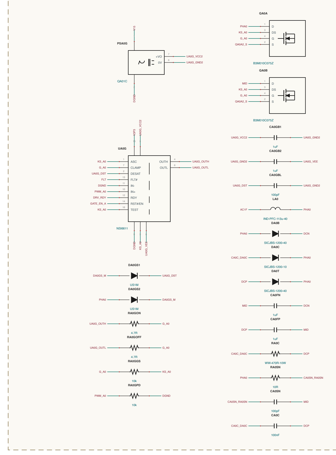
VIENNA-PFC / PHASE-A0
