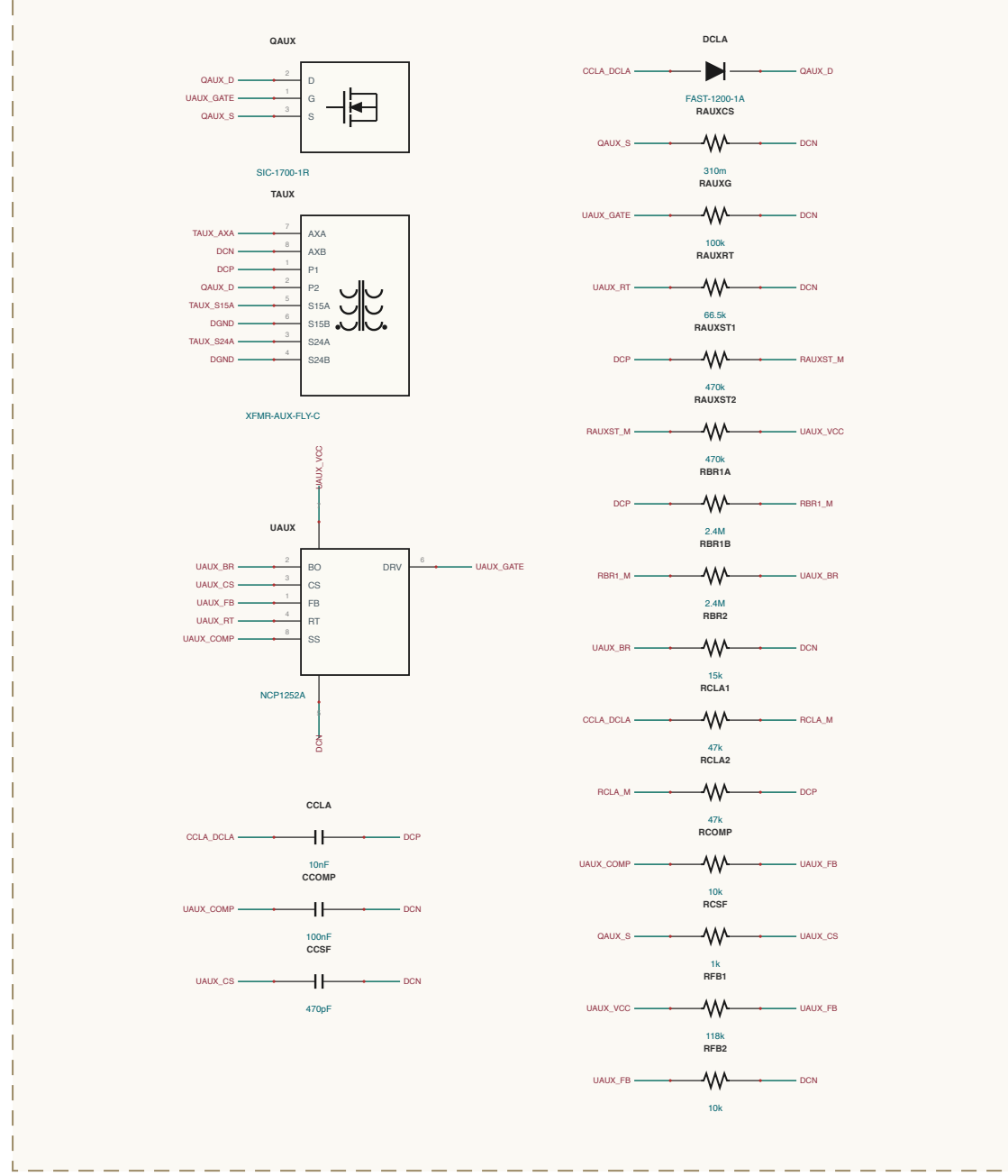
AUX-POWER / FLYBACK
